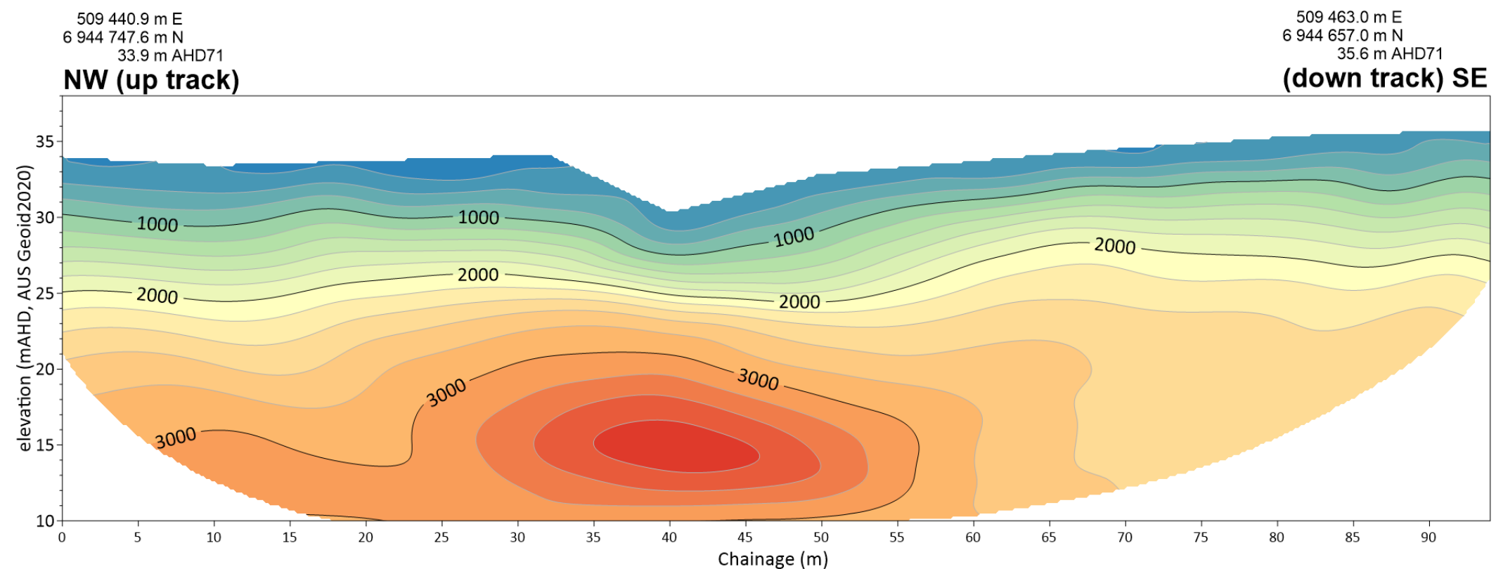
Seismic Line SR AU-GP 112
